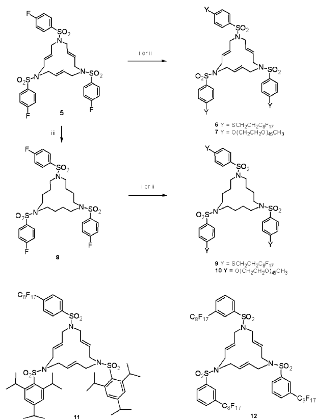
Scheme 1 Preparation of macrocycles; reagents and conditions. (i) To obtain 6 and 9 : \text{HSCH}_2\text{CH}_2\text{C}_8\text{F}_{17} , \text{Cs}_2\text{CO}_3 , n\text{-BuNCl} , THF, room temperature. (ii) To obtain 7 and 10 : \text{HO}(\text{CH}_2\text{CH}_2\text{O})_{45}\text{CH}_3 , NaH, THF, room temperature. (iii) Pd-C 10%, \text{PtO}_2 \cdot \text{H}_2\text{O} , THF, room temperature.
